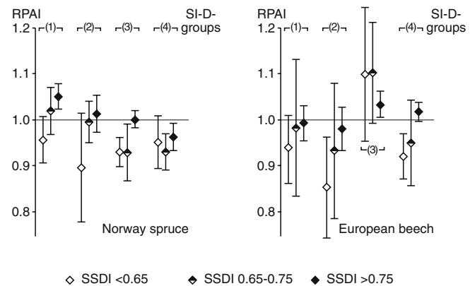
Fig. 8 RPAI (mean \pm 95% CI) for SSDI classes SSDI < 0.65 , 0.65–0.75 , and > 0.75 (empty, half filled, filled symbols, respectively). In order to reveal the effect of SI and D , stands are grouped (1) SI < SI_{50} , D < D_{50} , (2) SI < SI_{50} , D \geq D_{50} , (3) SI \geq SI_{50} , D < D_{50} , and (4) SI \geq SI_{50} , D \geq D_{50} . SI_{50} and D_{50} represent the 50% percentiles of SI and D in the dataset
