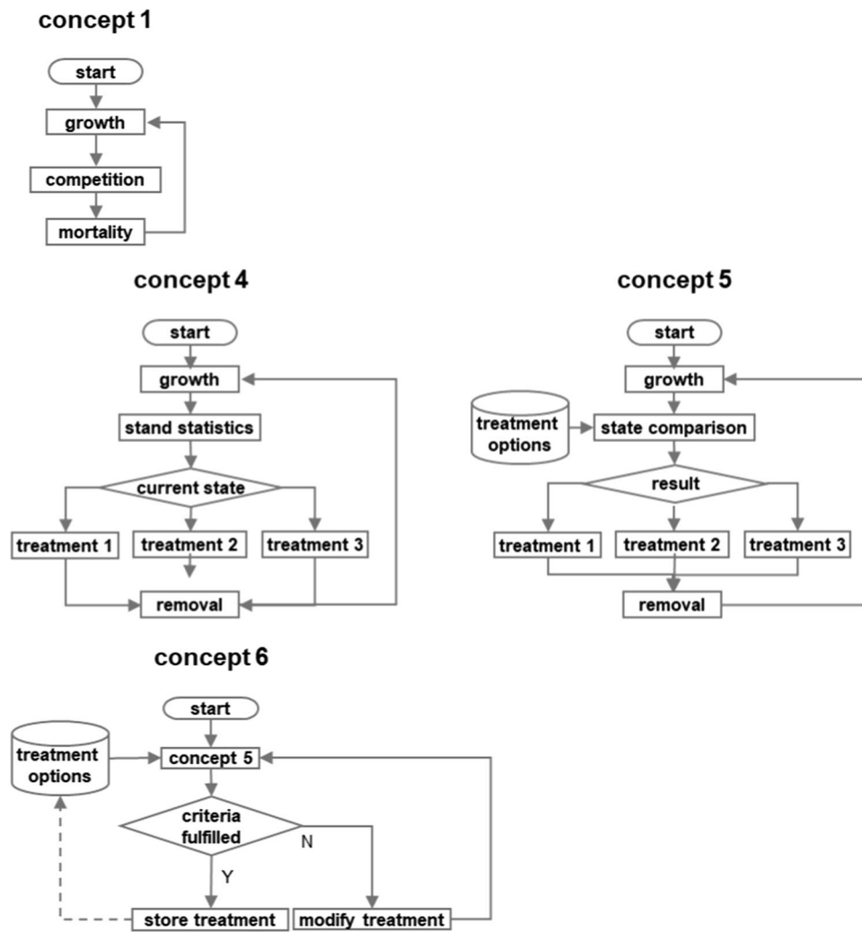
Fig. 4 Technical concepts of treatment implementation; concept 1 is typical for succession models, physiological or matrix models within their original field of application: thinning is an exclusive result of natural mortality; concept 2 is typical for models of concept 1 when extended for application in forestry: tree removal is an effect of thinning in addition, based on a thinning curve or a percentage of maximum density; concept 3 is typical for stand simulators when applied in education or consulting: the user selects from a group of alternative treatments, each time the system has come to a particular target state, e.g., given through stand age; concept 4 is typical for simulators
