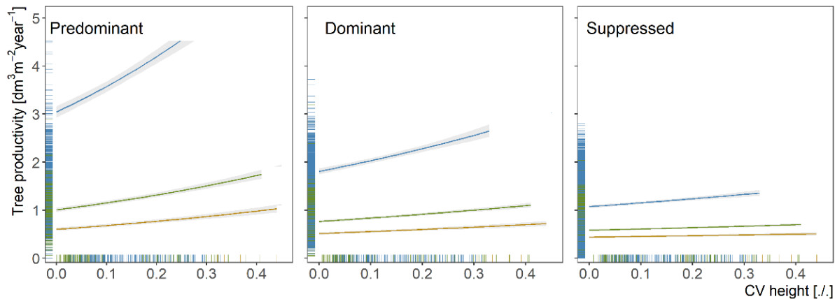
Figure 5. Productivity of oak trees as a function of coefficient of variation of tree heights and age for predominant ( rel\_d > 0.9 ), dominant ( rel\_d < 0.9 and > 0.7 ) and suppressed ( rel\_d < 0.7 ) oaks in monospecific stands; rugs on the x-and y-axis indicate the observed values of cvh and tree productivity, respectively; all other variables were set to their mean.
