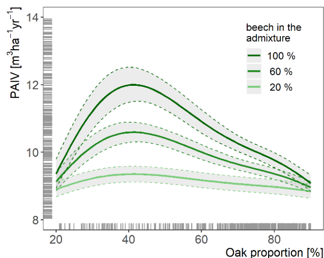
Figure 3. Non-linear smooth functions (GAMM) of stand productivity for mixed oak stands as a function of oak proportions and proportion of beech in the admixture; rugs on the x-and y-axis indicate the observed values of oak proportions and stand productivity, respectively; for the underlying model statistics we refer to the supplementary material (Table S4).
